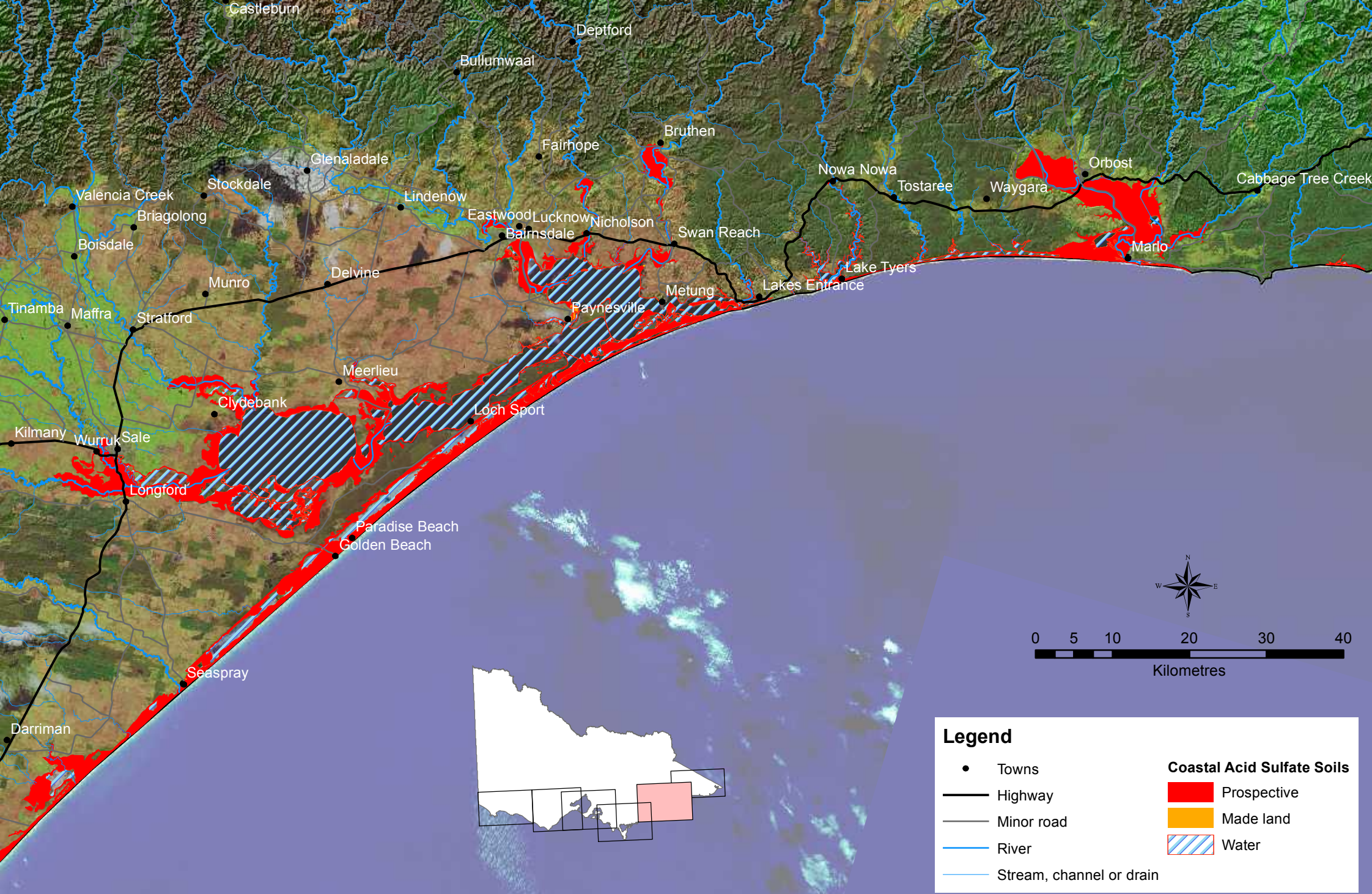
Coastal Acid Sulfate Soils Distribution - Map 5 for the Gippsland Lakes of Victoria
