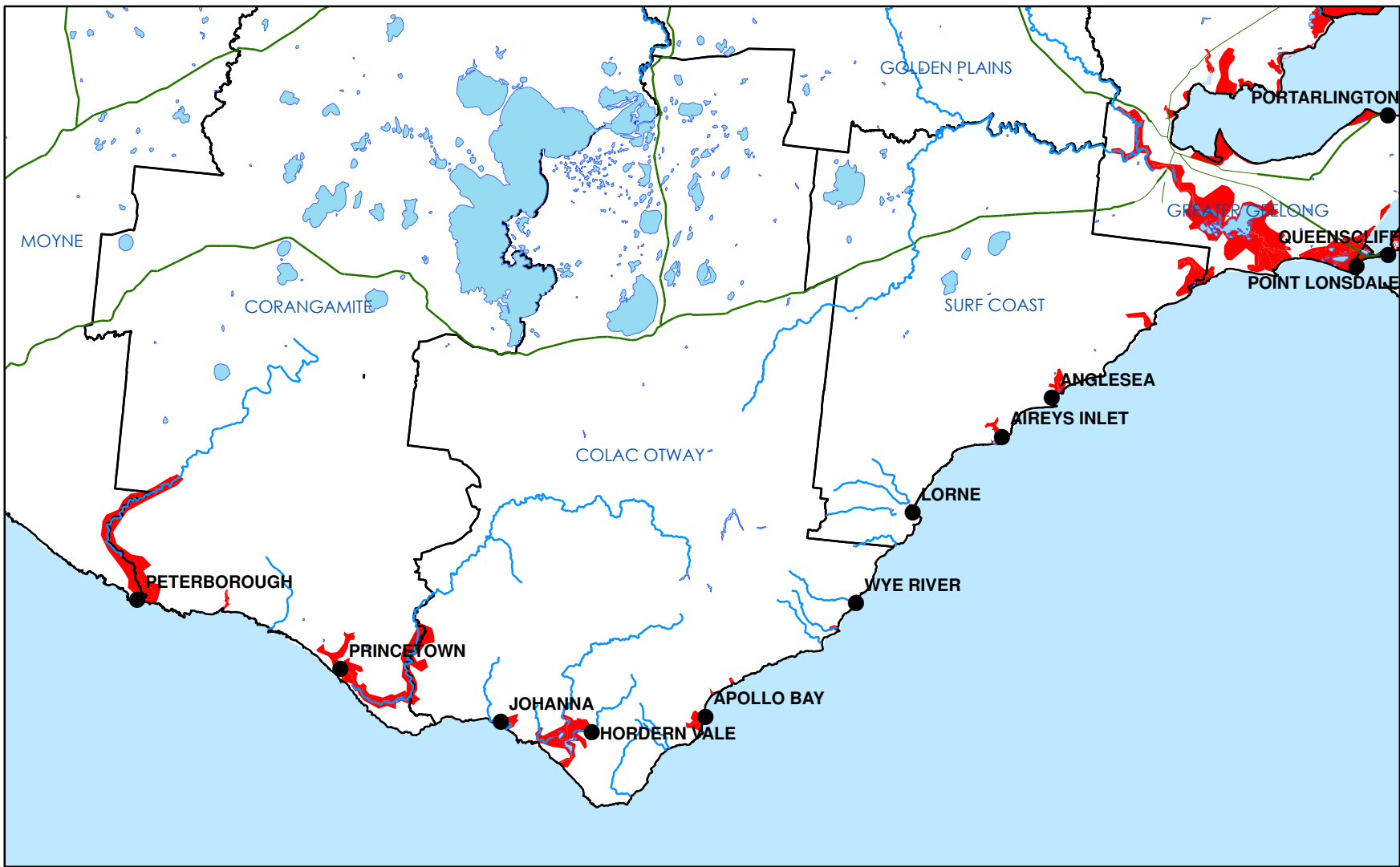
Map 2 West Coast Prospective Land: land that has the potential to contain Coastal Acid Sulfate Soils
