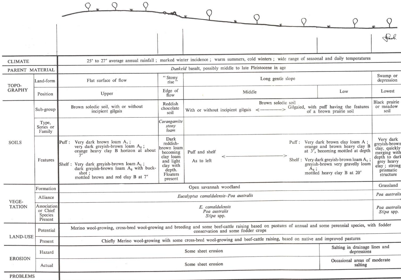
Fig.39 Land-system diagram
