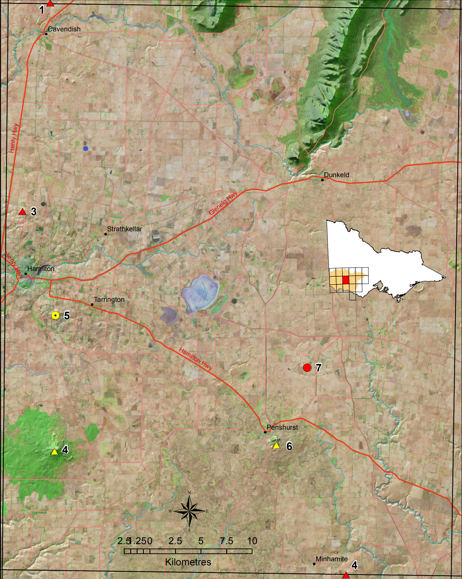
Hamilton 1:100 000 mapsheet Eruption Points of the Newer Volcanics (Rosengren)
