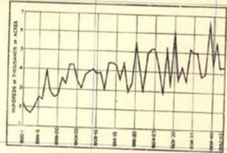
GRAPH SHOWING TOTAL ACREAGE UNDER OATS 1890.1-1942.3
