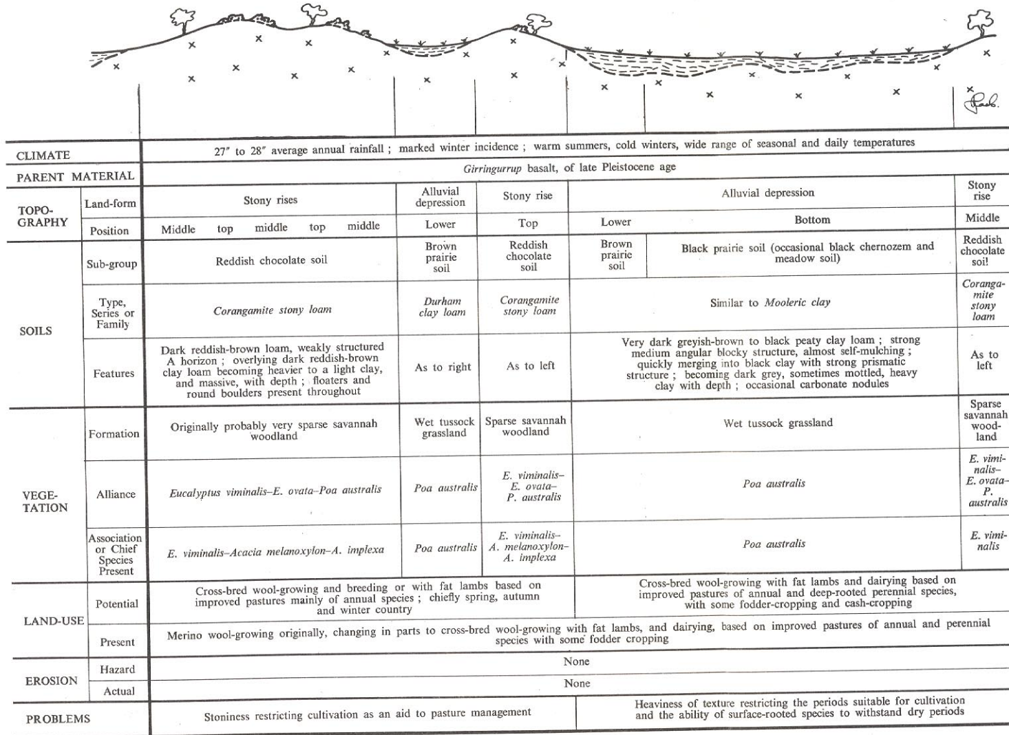
Fig. 40 Land-system diagram
