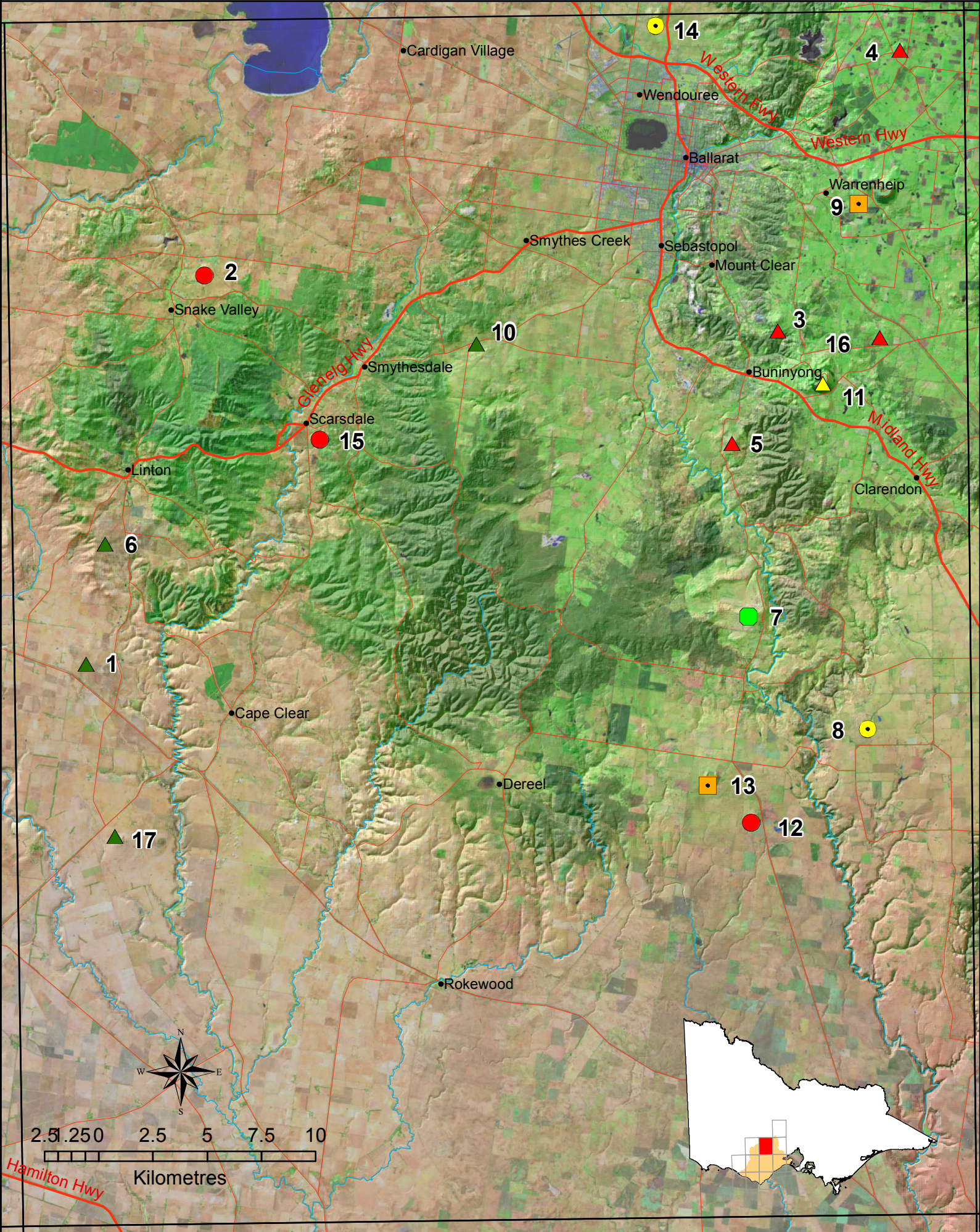
Ballarat 1:100 000 mapsheet Eruption Points of the Newer Volcanics (Rosengren)
