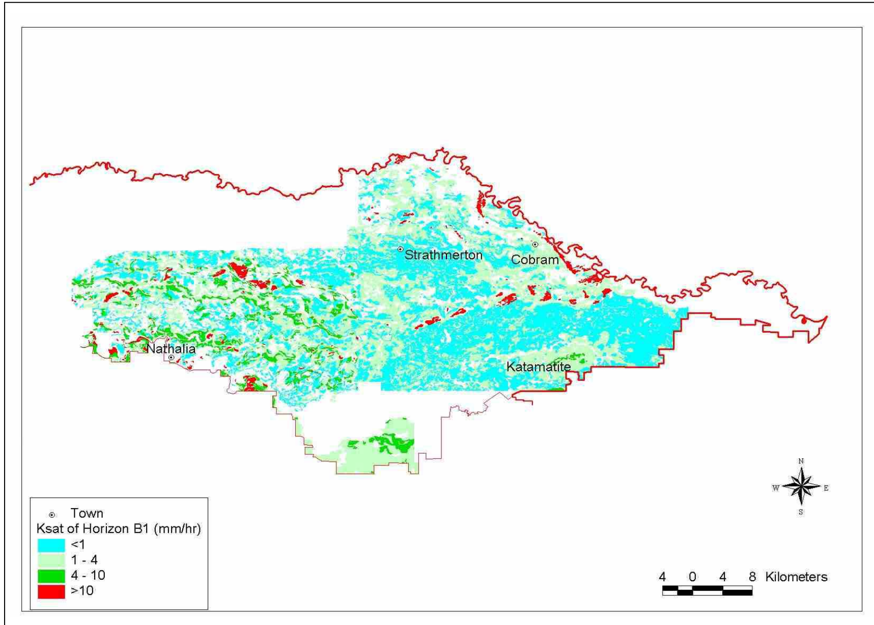
Figure 4.1 Saturated Hydraulic Conductivity of Horizon B1 – MV Irrigation Area
