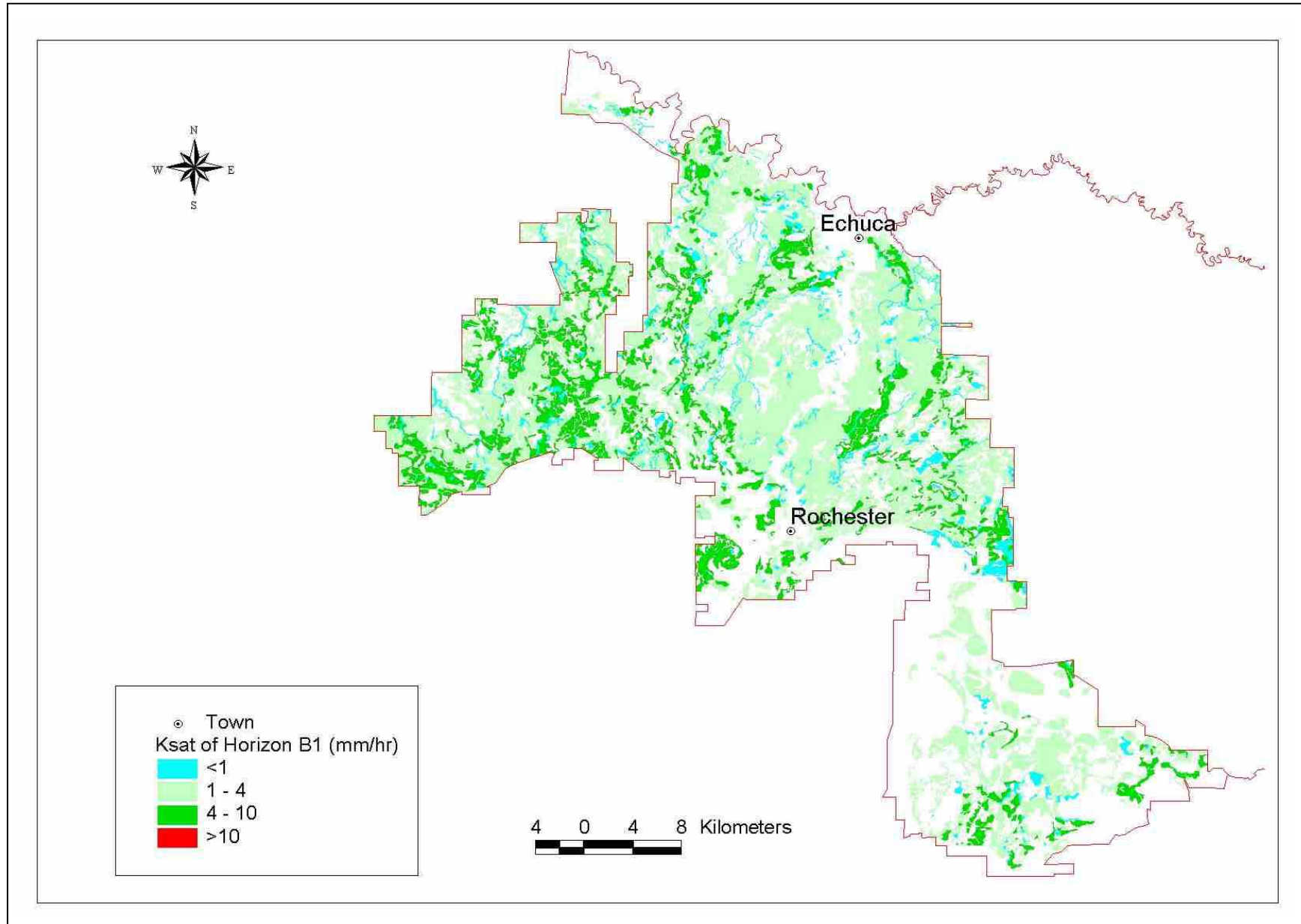
Figure 4.3 Saturated Hydraulic Conductivity of Horizon B1 – RC Irrigation Area
