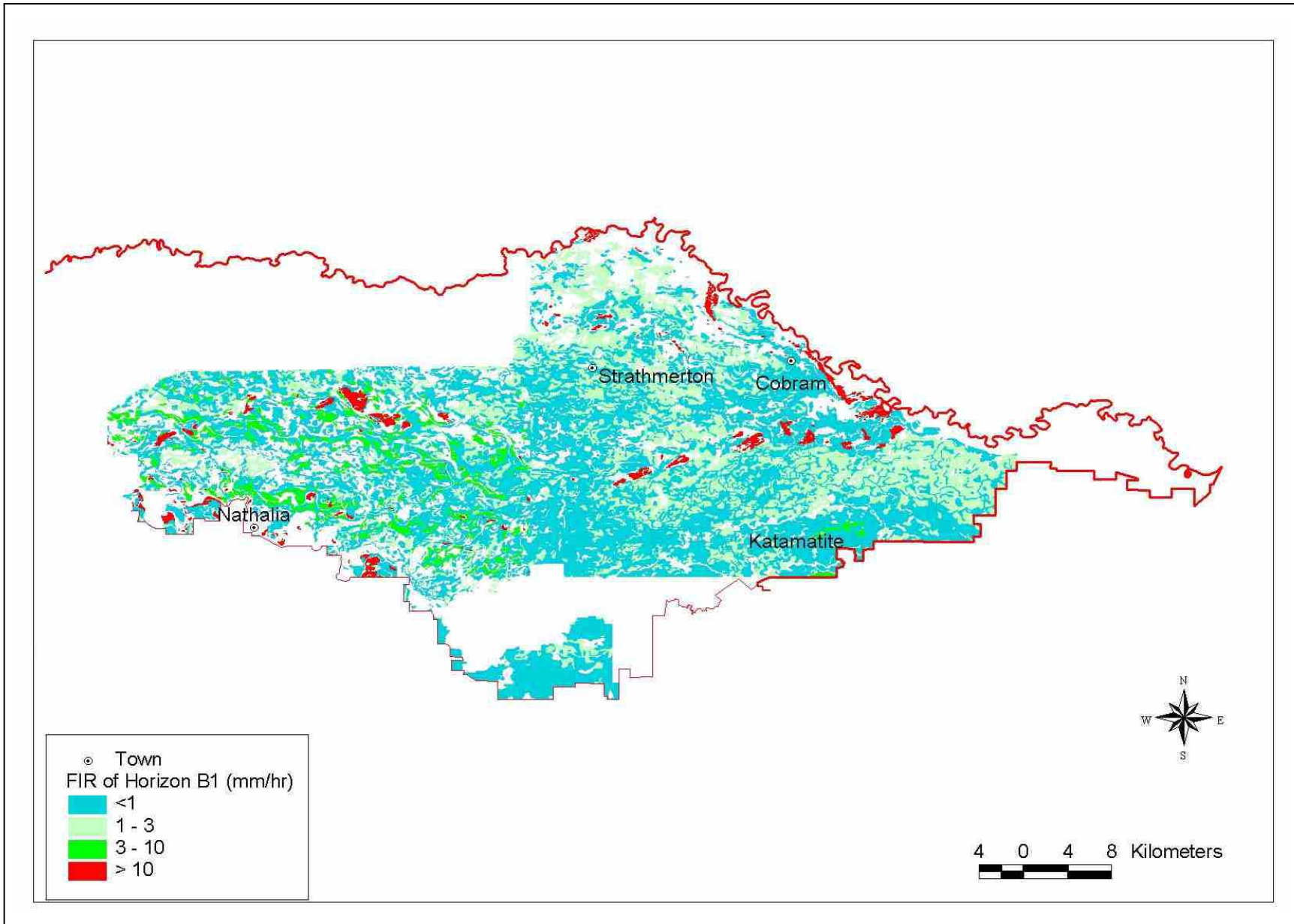
Figure 5.1 Final Infiltration Rate of MV Irrigation Area
